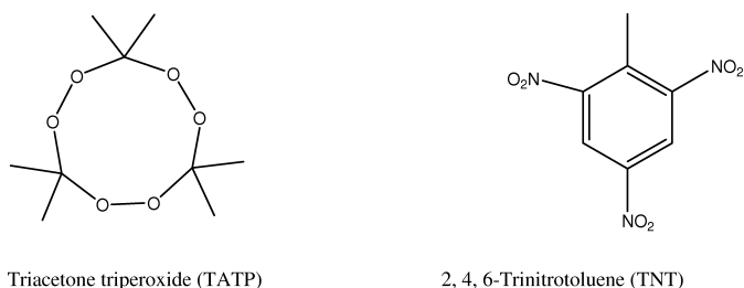
Triacetone triperoxide (TATP)
