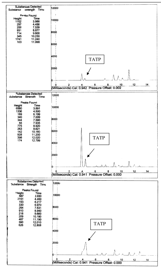
FIG. 8—Plasmagrams (N-mode) from Asian hair exposed to TATP vapor for 3 days. (A) Hair (~0.05 g) placed directly in the vapor desorption unit of the IMS. (B) A swab from the TATP contaminated hair (mg) placed directly in the vapor desorption unit of the IMS. (C) Acetonitrile extract (100 µL) of a portion of TATP contaminated hair (~0.05 g) placed on N-mode sample trap and inserted into vapor desorption unit of IMS.
